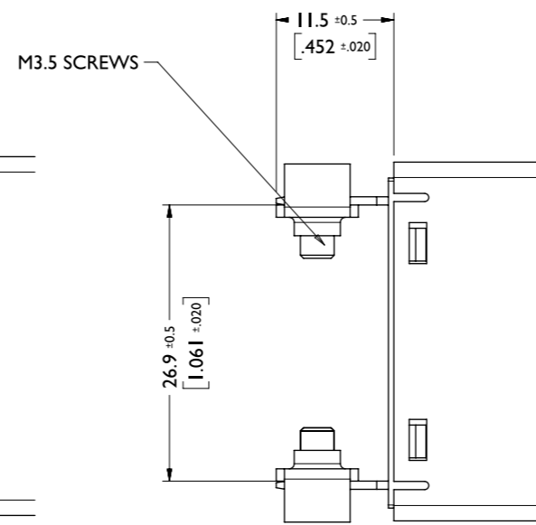
CLAMP TERMINAL
