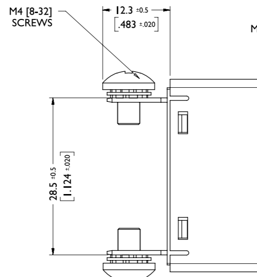
SCREW TERMINAL
